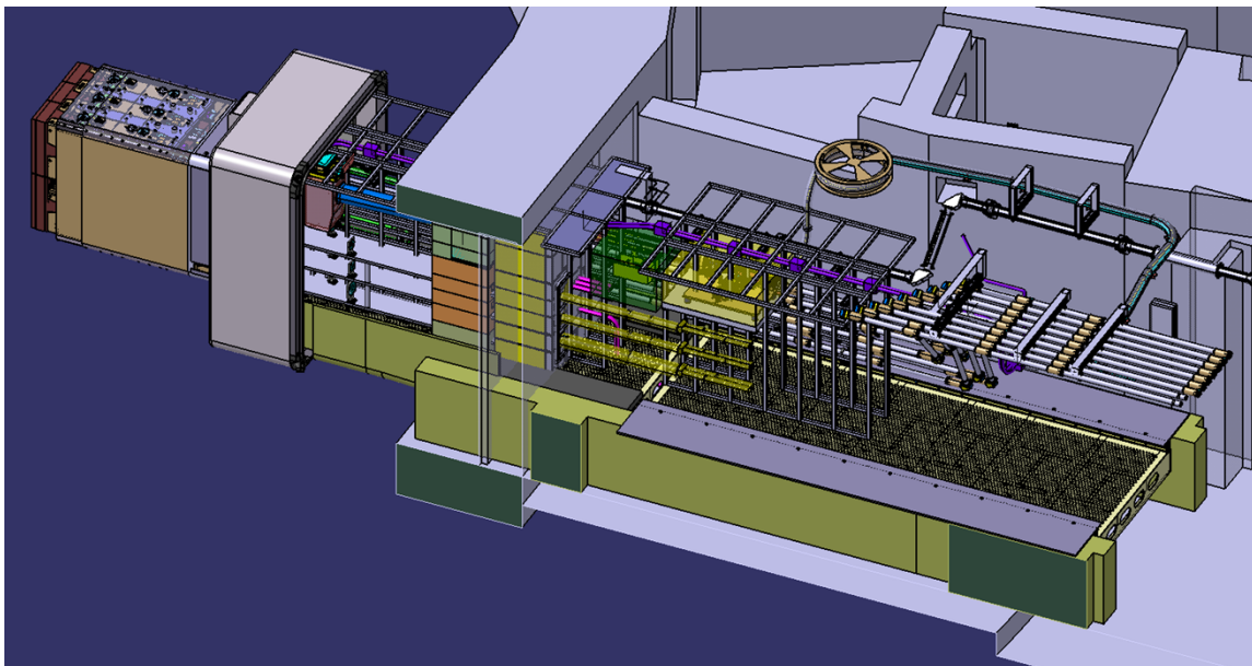
Figure 1. General layout of port interspace/ cell in Equatorial Port #12.
